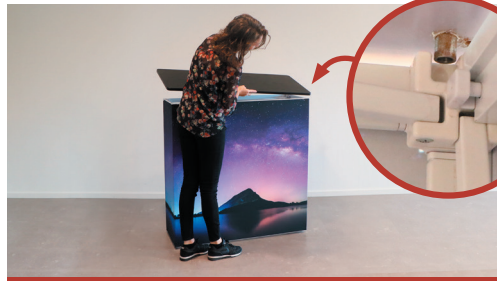
16. Place the tabletop on top of the frame, so the aluminium buttons fit the gaps in the frame.
